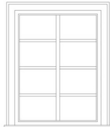
TYPICAL WINDOW TRIM DETAIL
